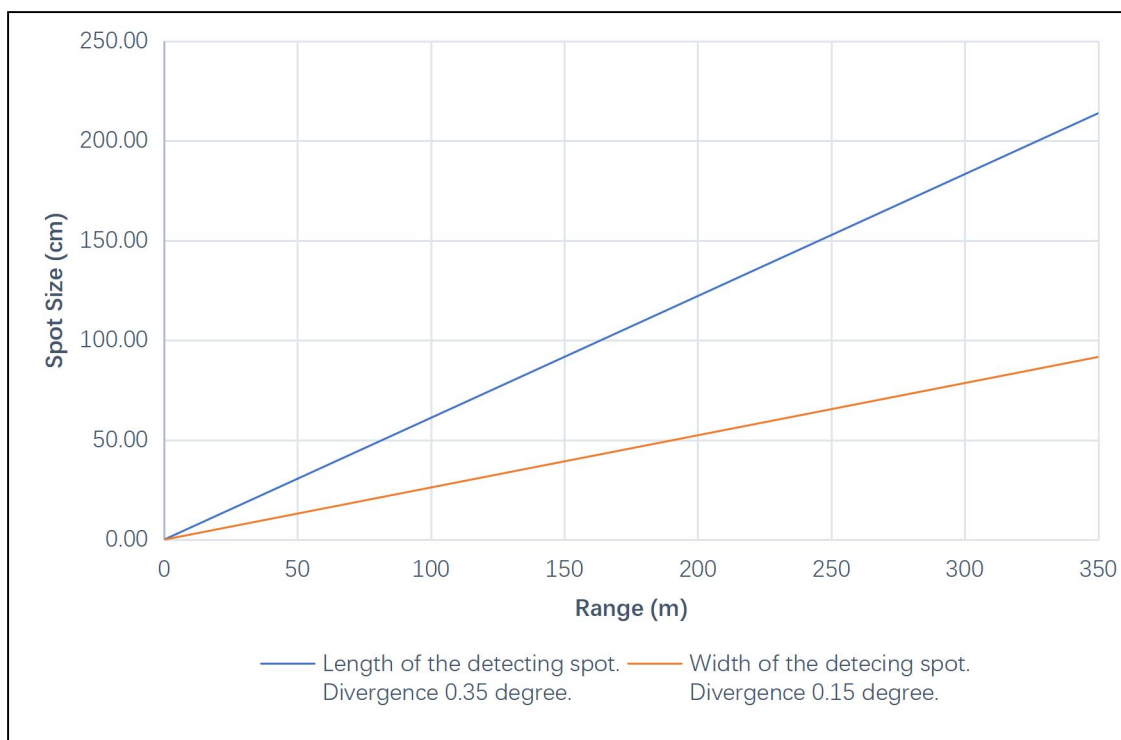
Figure 5 Spot size of TF350 at different ranges
