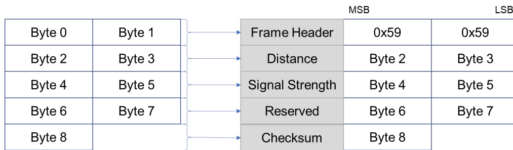
Figure 11 Data communication: User protocol frame format of UART
