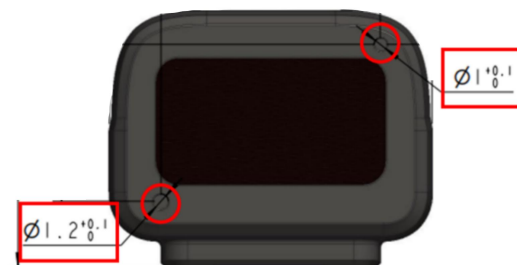
Figure. 4: Diagram of TF-NOVA installation hole
