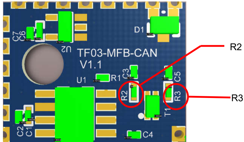
Figure 10 Resistances needed to be removed from board for CAN Bus
