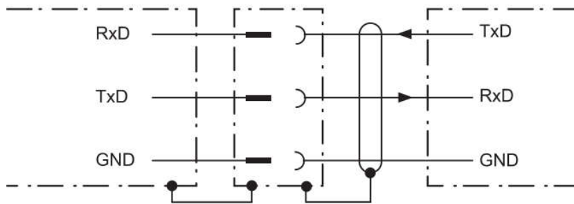
Figure 7 Wiring of the UART interface
