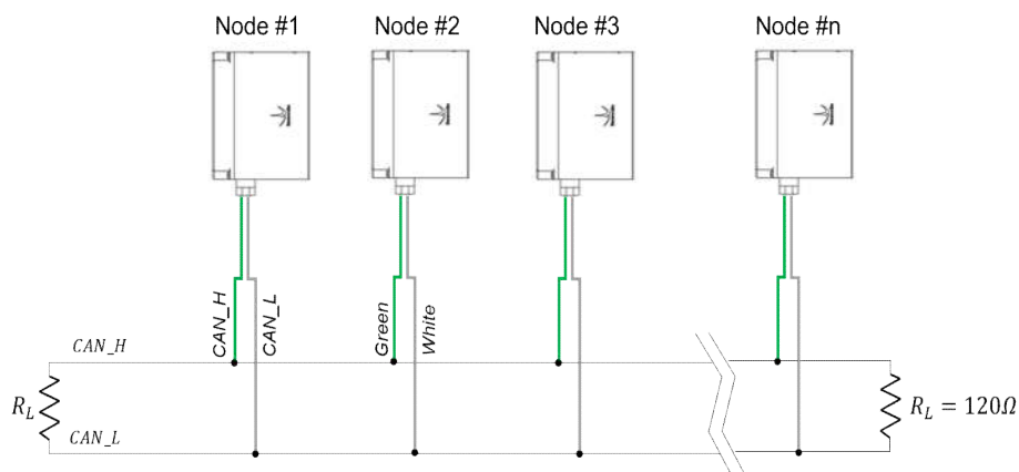
Figure 9 CAN networking of TF350
