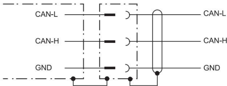
Figure 8 Wiring of the CAN interface
