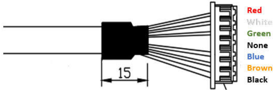
Figure 6 Male connector, Molex SD-51021-007 1.25 W/B-7Pin
