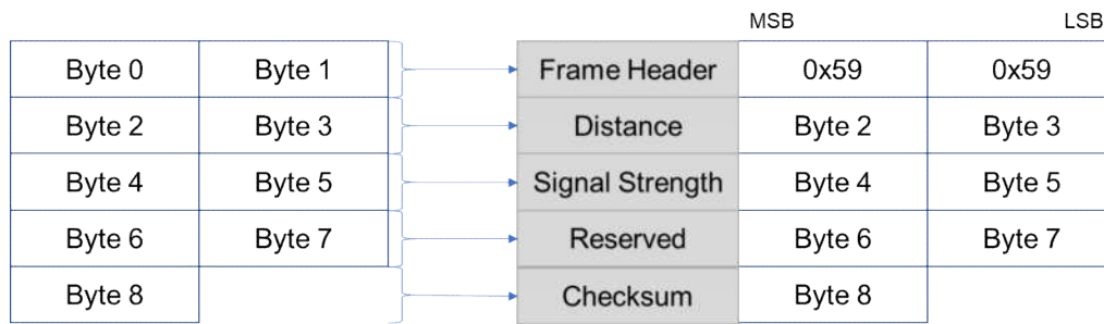
Figure 11 Data communication: User protocol frame format of UART
