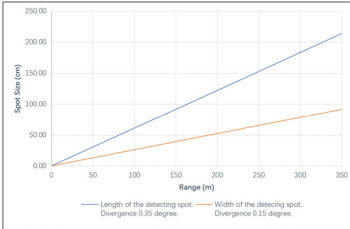
Figure 5 Spot size of TF350 at different ranges
