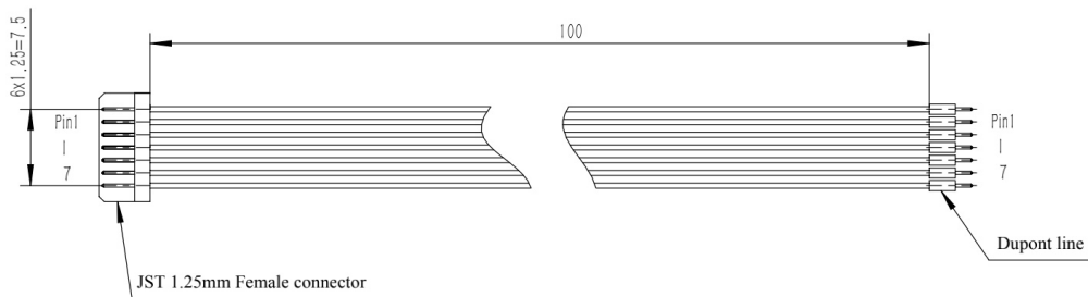
Figure 14 Extension cord for test
